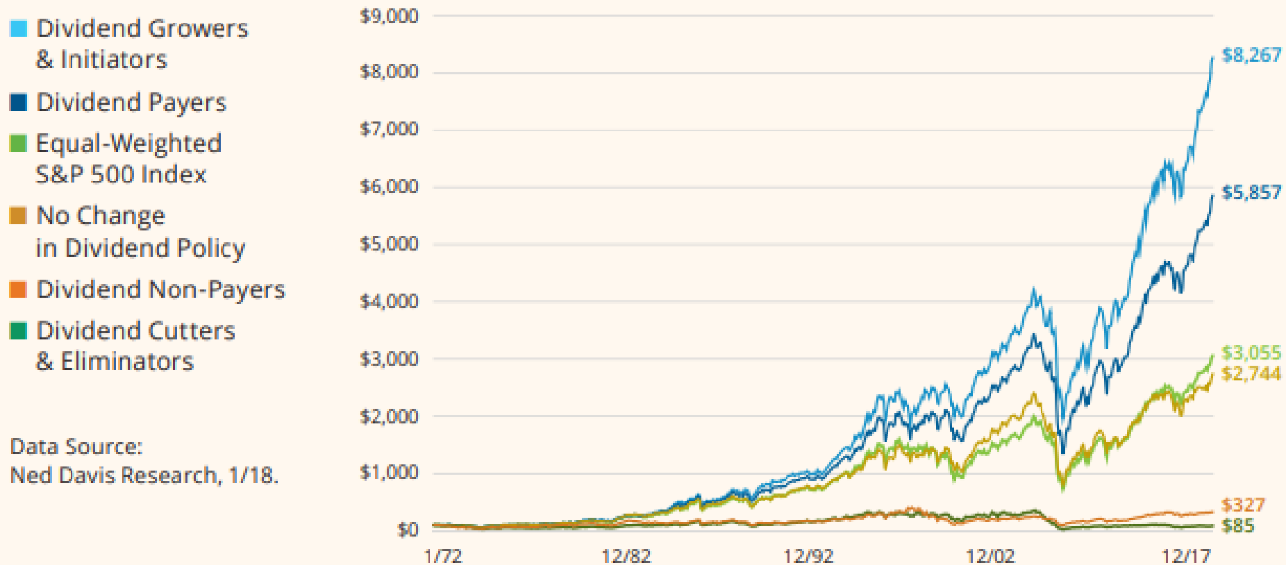
Returns of S&P 500 Index Stocks by Dividend Policy: Growth of $100 (1/1972-12/2017)
